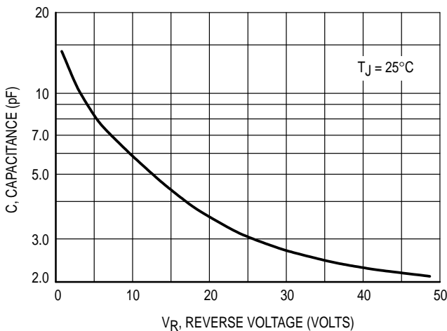
Figure 10. Typical Capacitance
