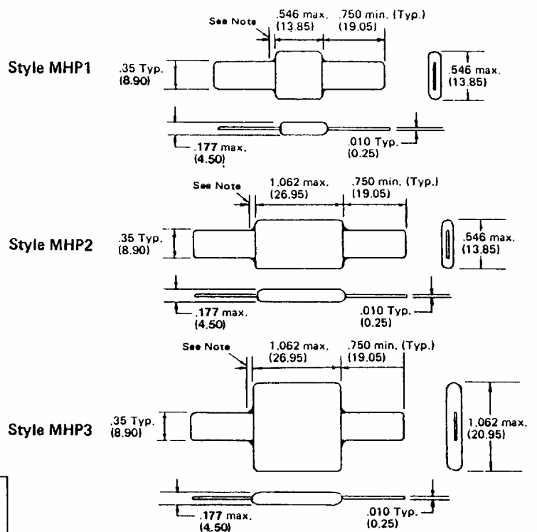
All dimensions in inches (mm)
