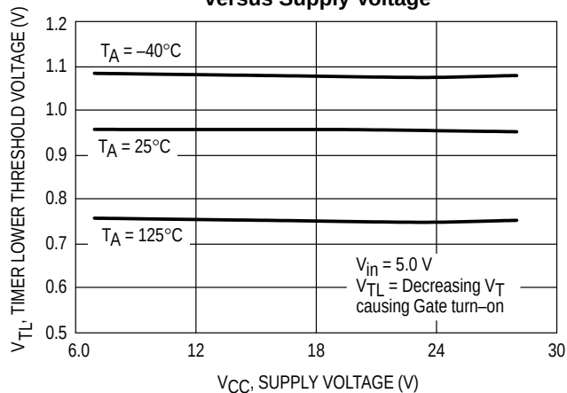
Figure 13. Timer Lower Threshold Voltage versus Supply Voltage
