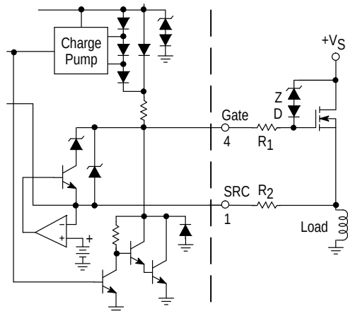
Figure 36. Overvoltage Protection of FET
