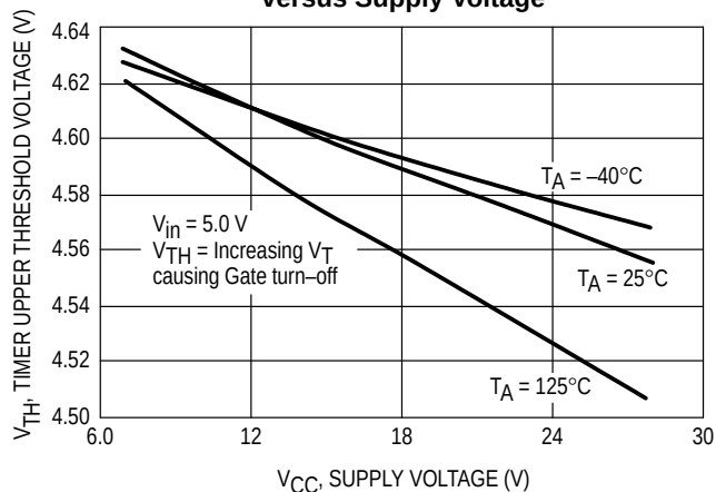
Figure 11. Timer Upper Threshold Voltage versus Supply Voltage
