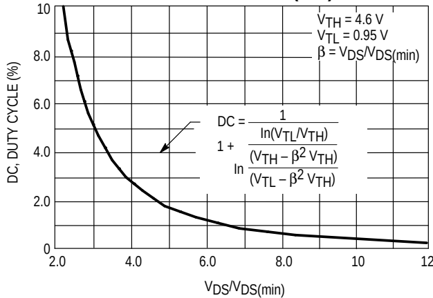
Figure 30. MC33091A Duty Cycle versus V_{DS} / V_{DS(min)}
