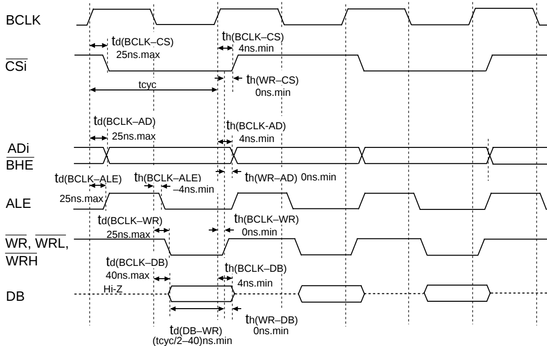
Figure 21-4. V CC = 5V timing diagram
