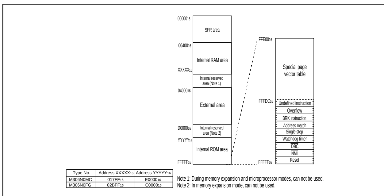
Figure 2-1. Memory map
