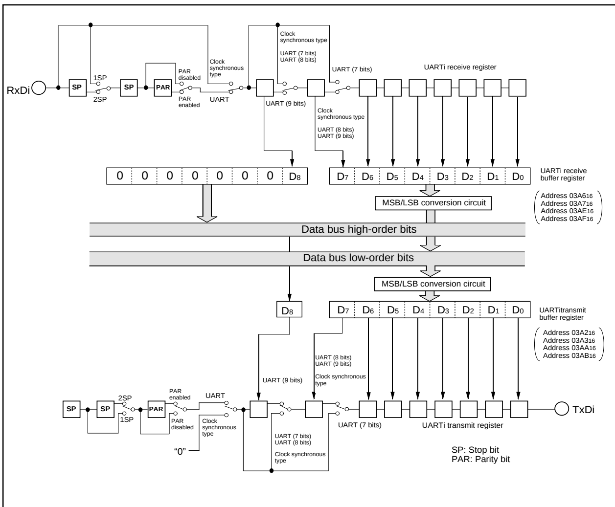
Figure 12-2. Block diagram of UART i (i = 0, 1) transmit/receive unit
