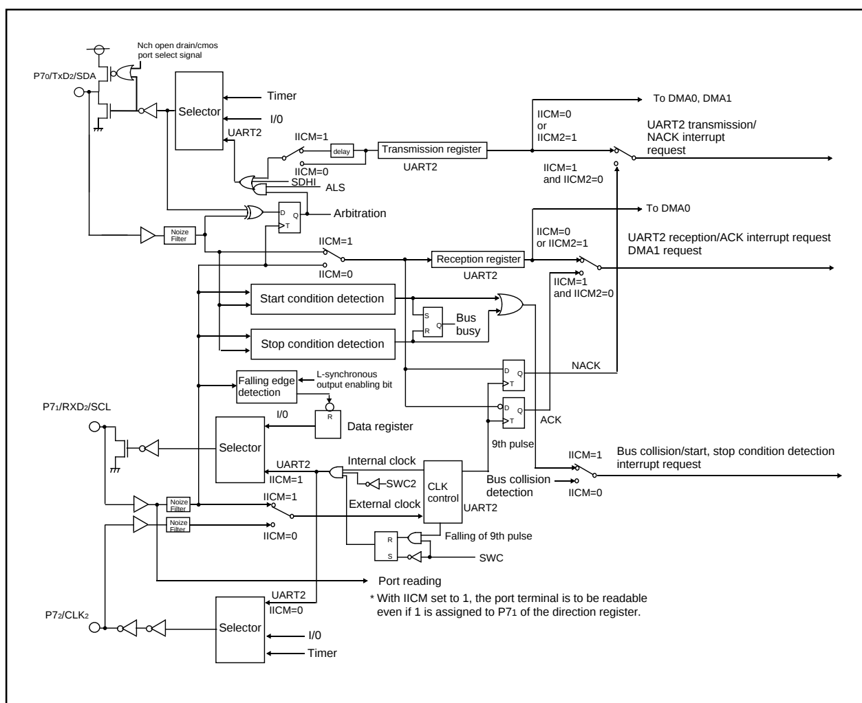
Figure 13-15. Functional block diagram for I²C mode
