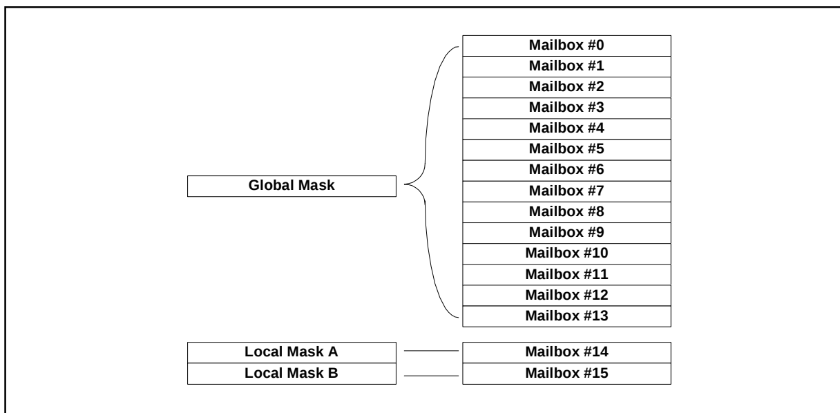
Figure 18-12. Mask assignment
