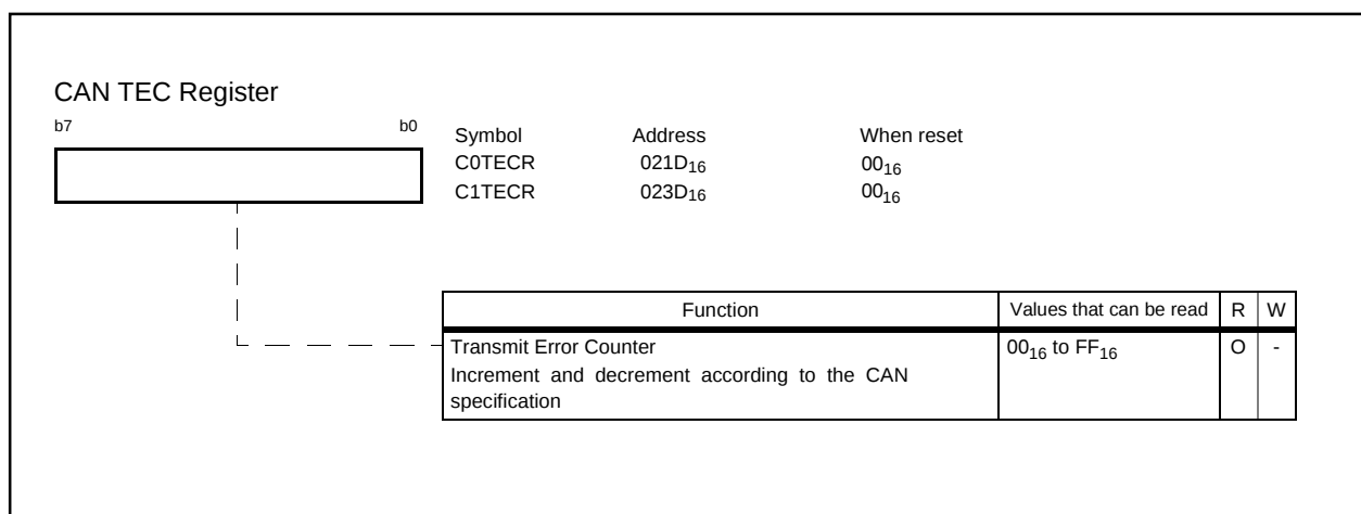
Figure 18-20. Structure of CAN TEC register (Transmit error counter)
