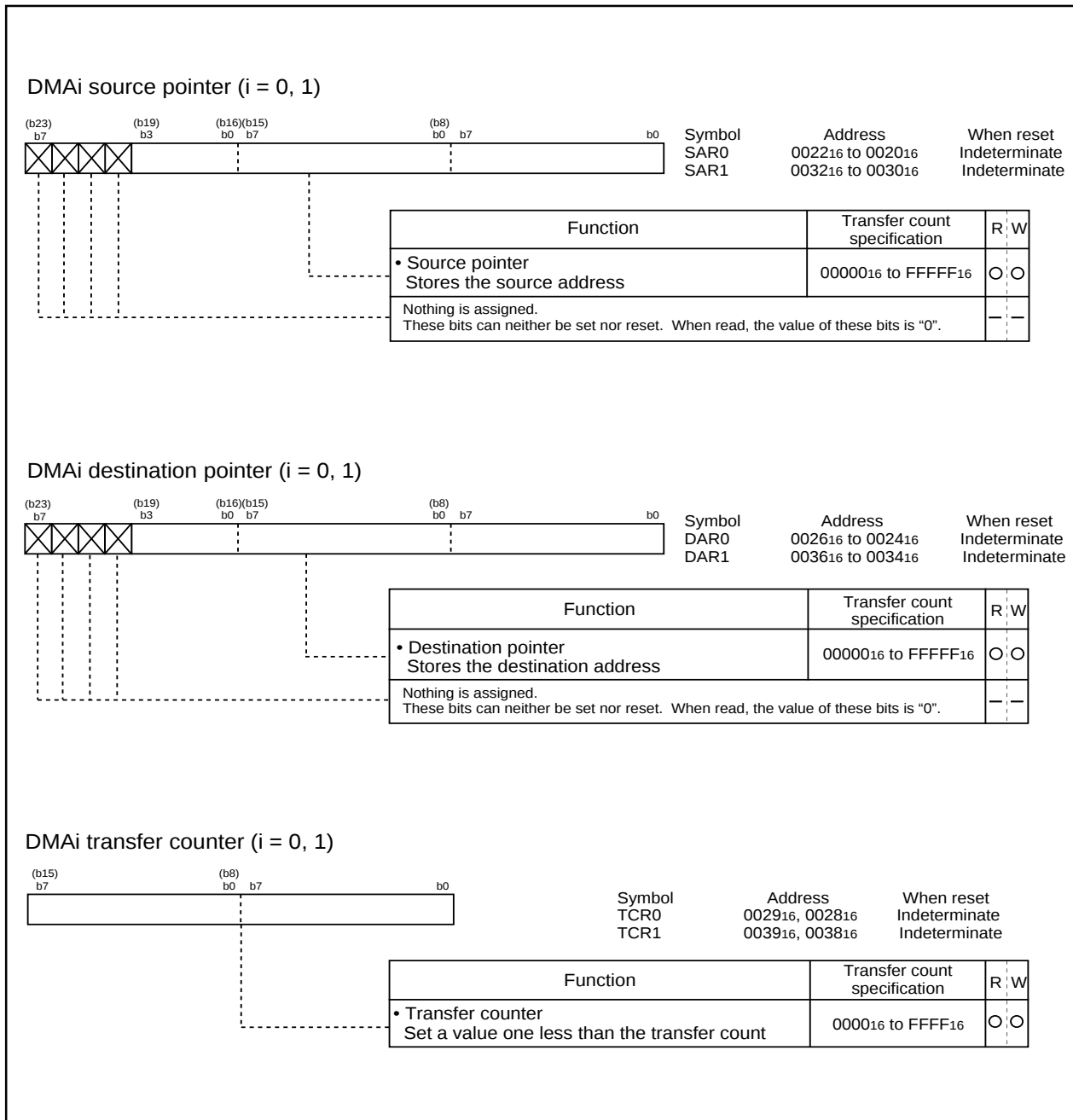
Figure 7-4. DMAC register (3)
