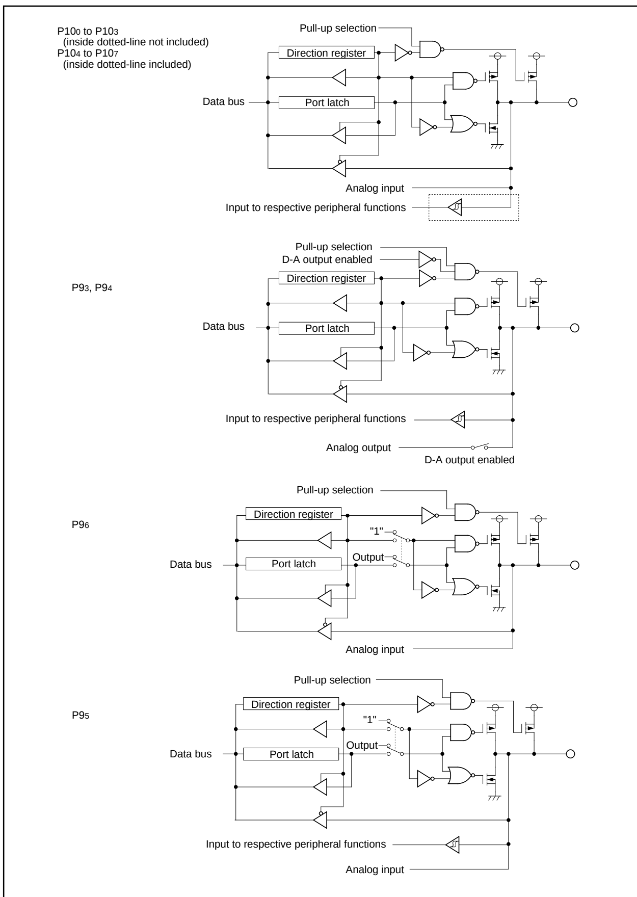
Figure 19-3. Programmable I/O ports (3)
