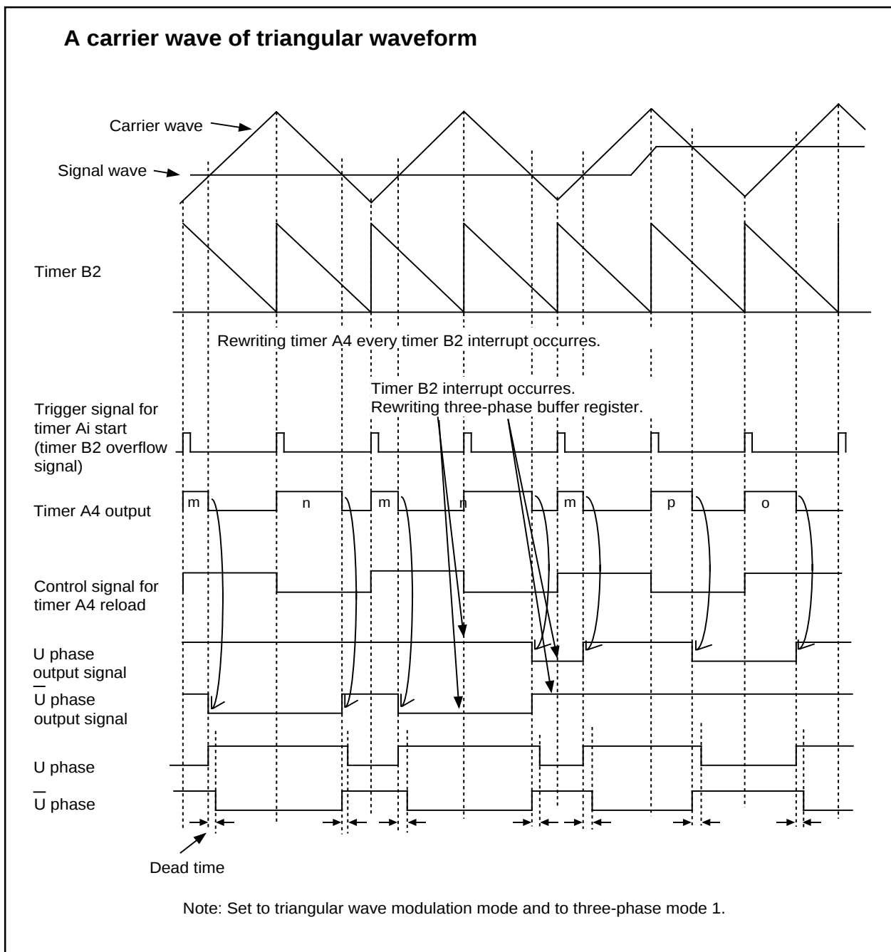
Figure 11-7. Timing chart of operation (2)
