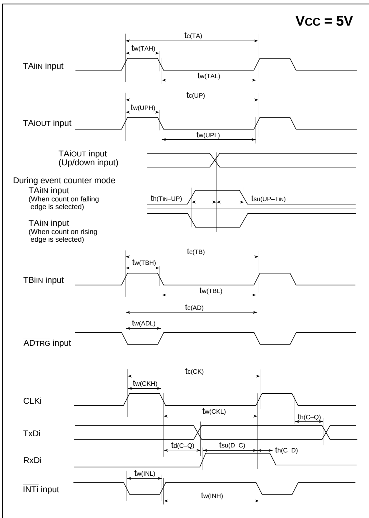
Figure 21-2. Vcc = 5V timing diagram
