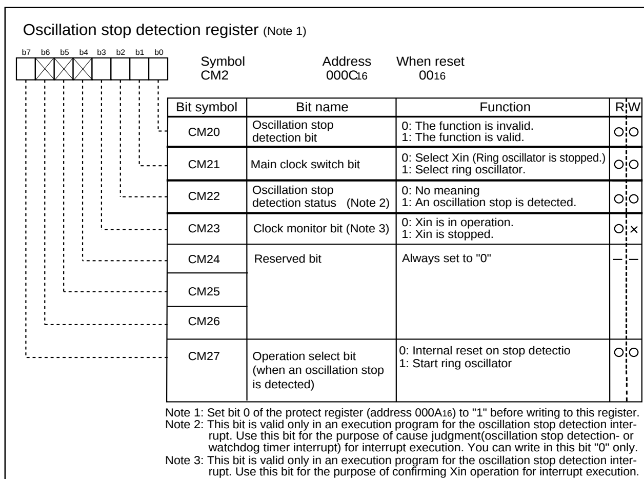
Figure 5-9. Structure of the oscillation stop detection register
