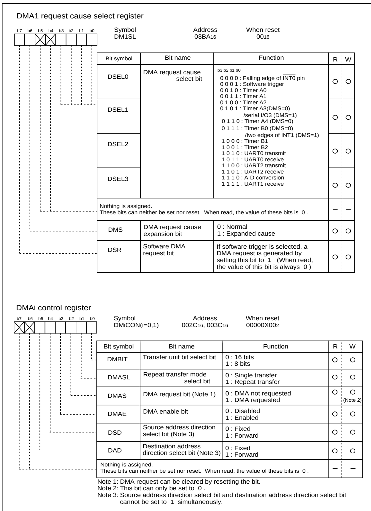
Figure 7-3. DMAC register (2)
