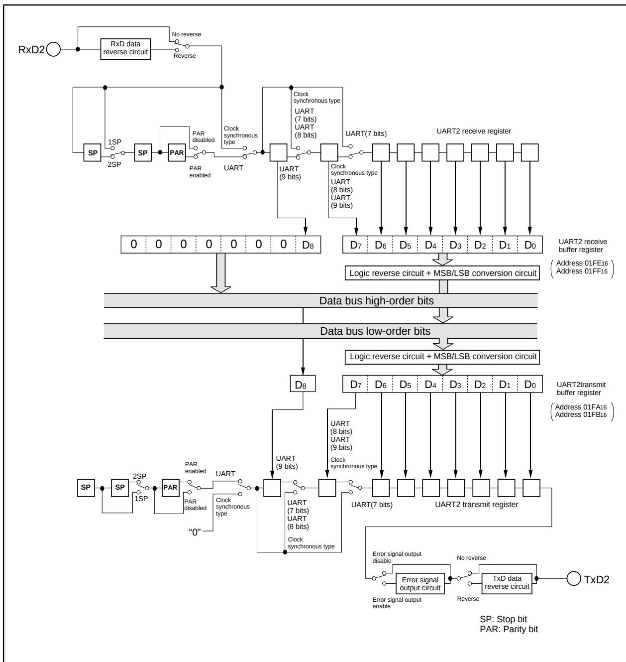
Figure 12-3. Block diagram of UART2 transmit/receive unit
