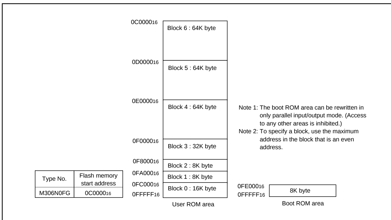
Figure 22-3. Block diagram of on-chip flash memory
