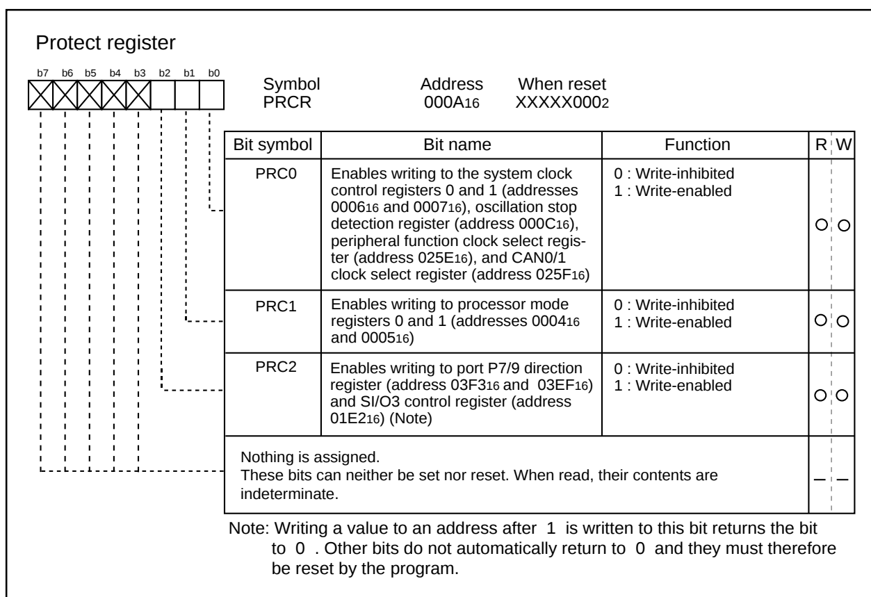
Figure 3-9. Protect register
