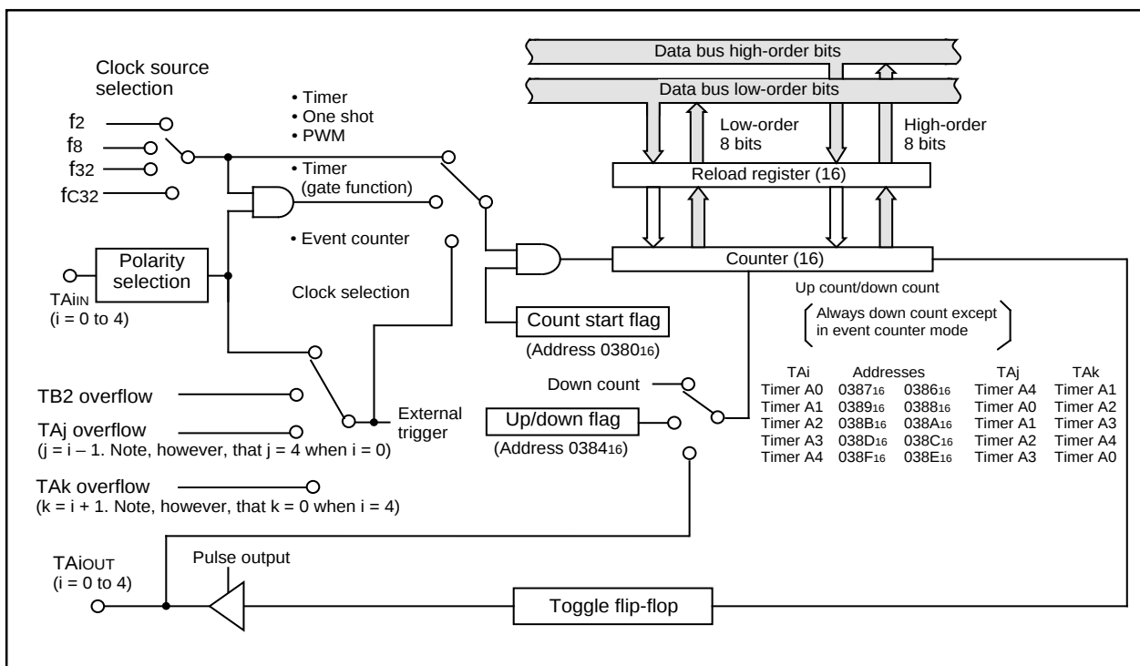
Figure 9-3. Block diagram of timer A
