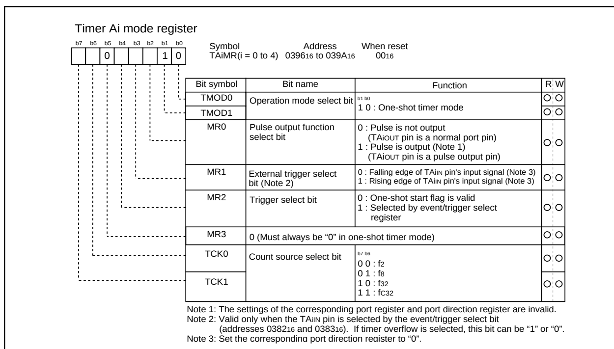
Figure 9-10. Timer Ai mode register in one-shot timer mode
