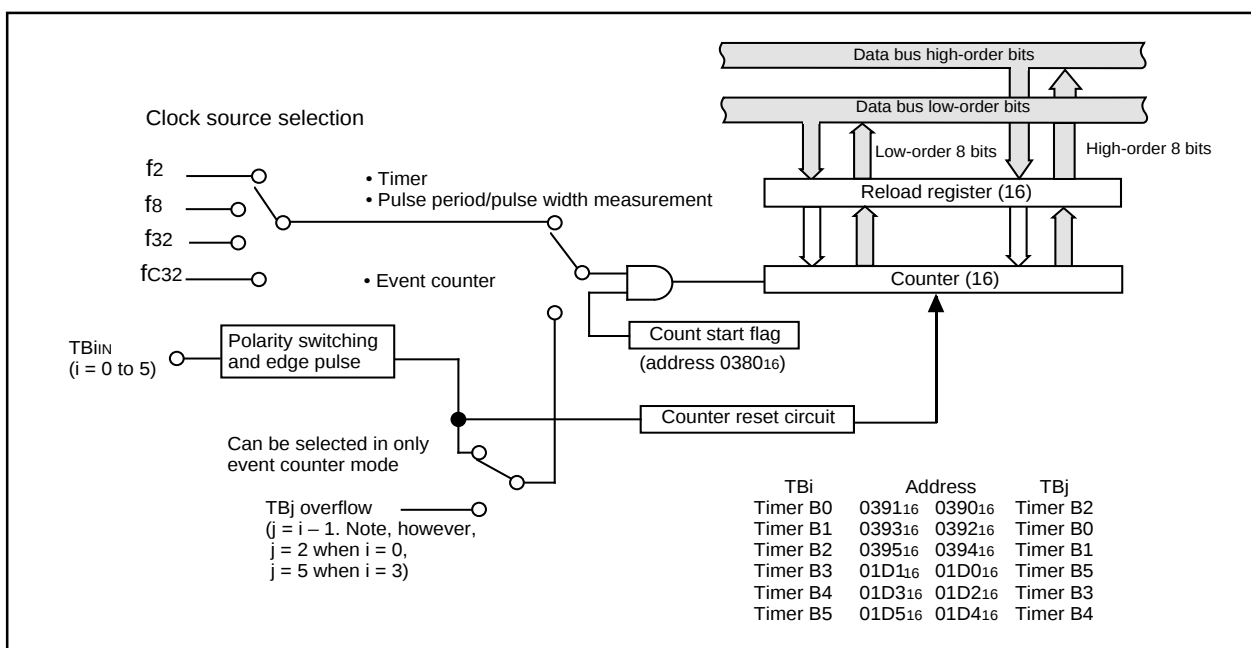
Figure 10-1. Block diagram of timer B
