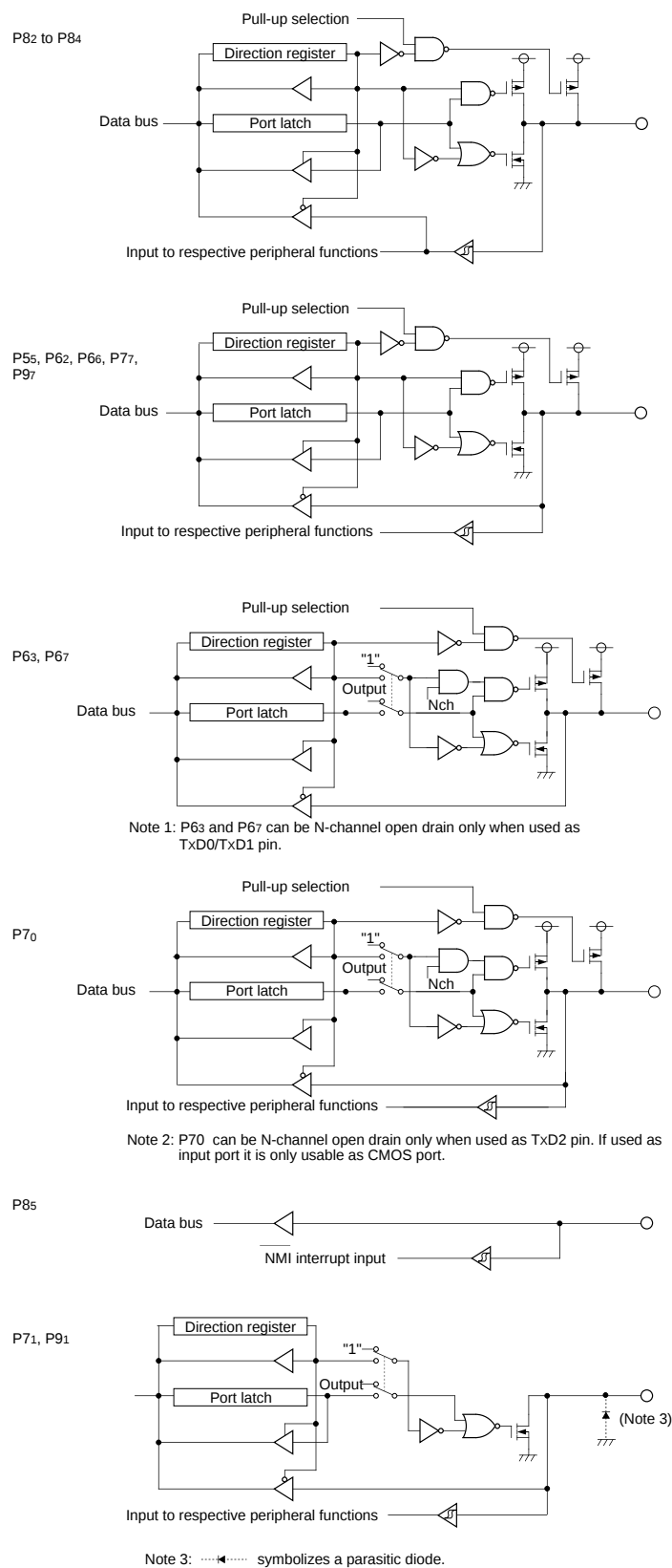
Figure 19-2. Programmable I/O ports (2)
