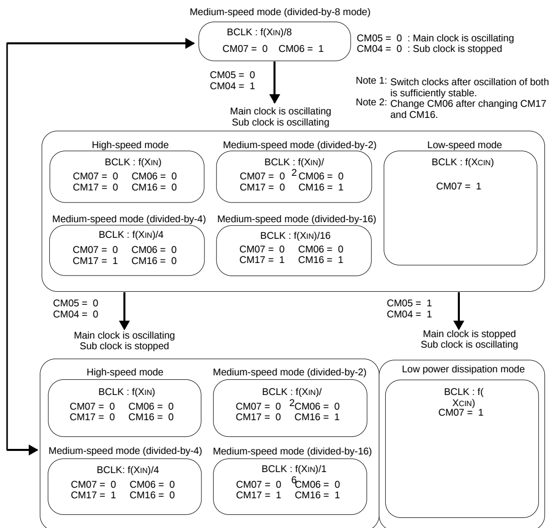
Figure 5-7. State transition diagram of power control mode
