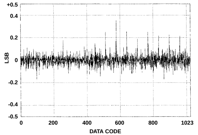
FIGURE 5. DIFFERENTIAL NON-LINEARITY
