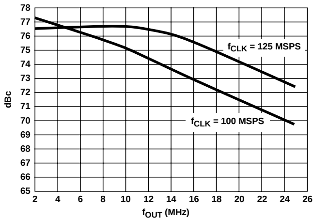
FIGURE 10. SPURIOUS FREE DYNAMIC RANGE (±1MHz WINDOW) vs FREQUENCY
