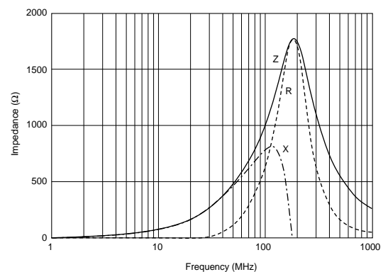
BLM18BD102SN1
