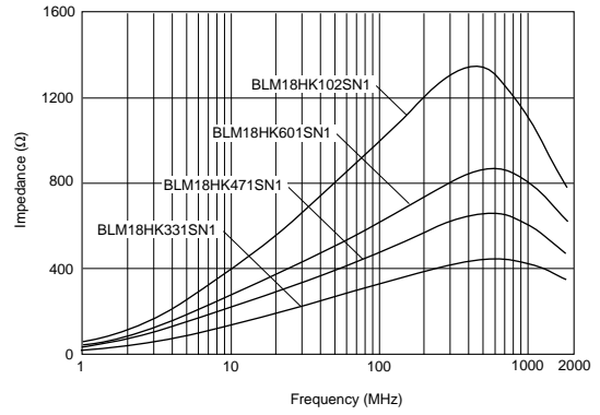
BLM18HK Series
