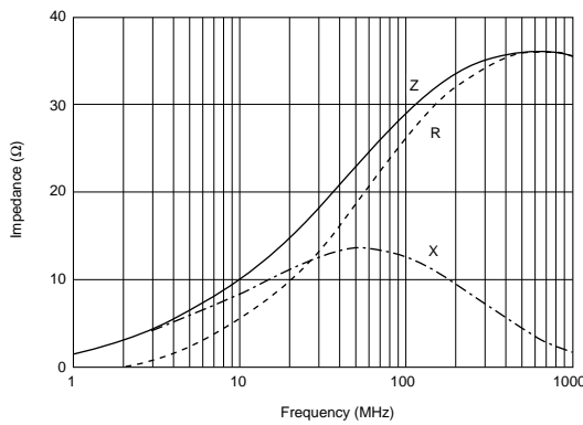
BLA31AG300SN4
