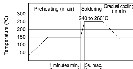
[Flow Soldering]
