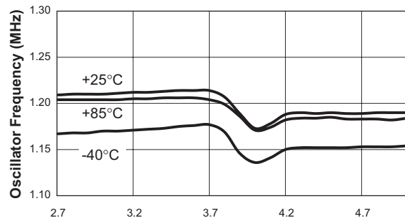
Oscillator Frequency vs. Supply Voltage
