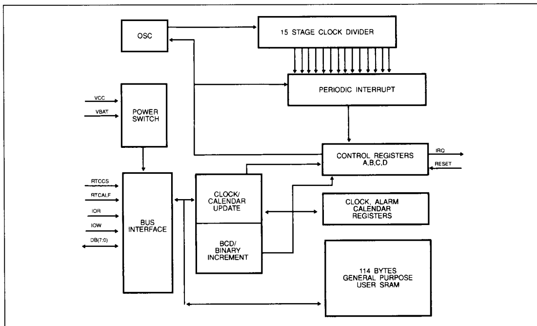
FIGURE 2-3. RTC BLOCK DIAGRAM
