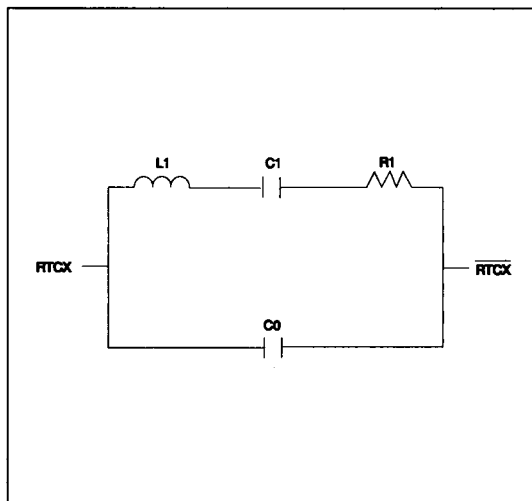
FIGURE 2-5. RTC CRYSTAL PARAMETERS
