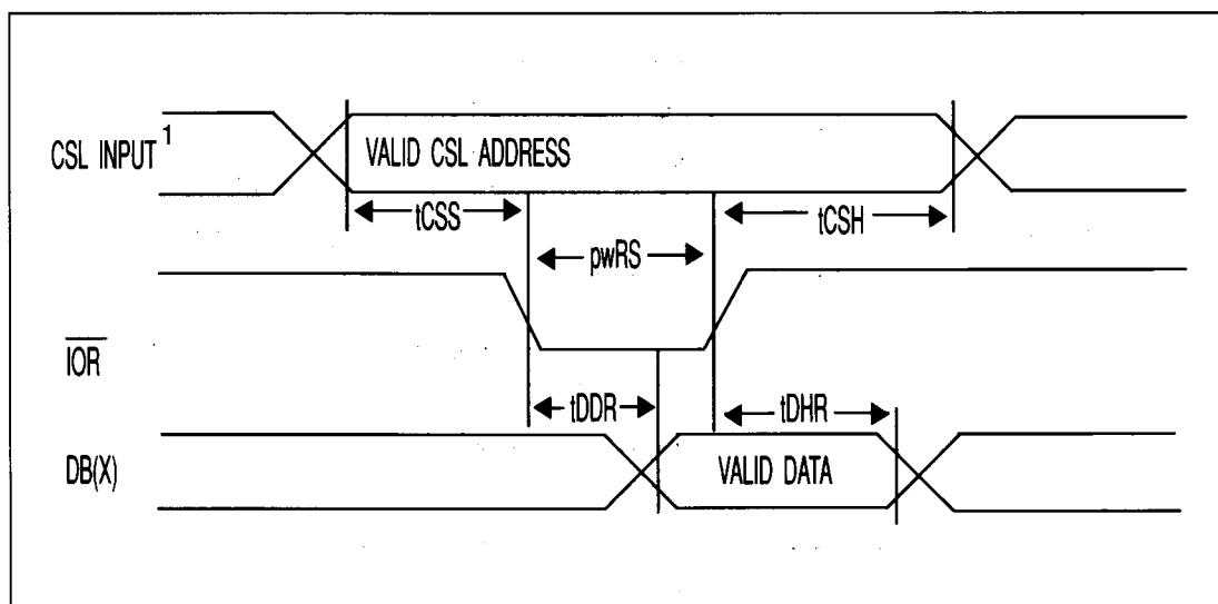
FIGURE 4-9. RTC AND RAM READ TIMING DIAGRAM
