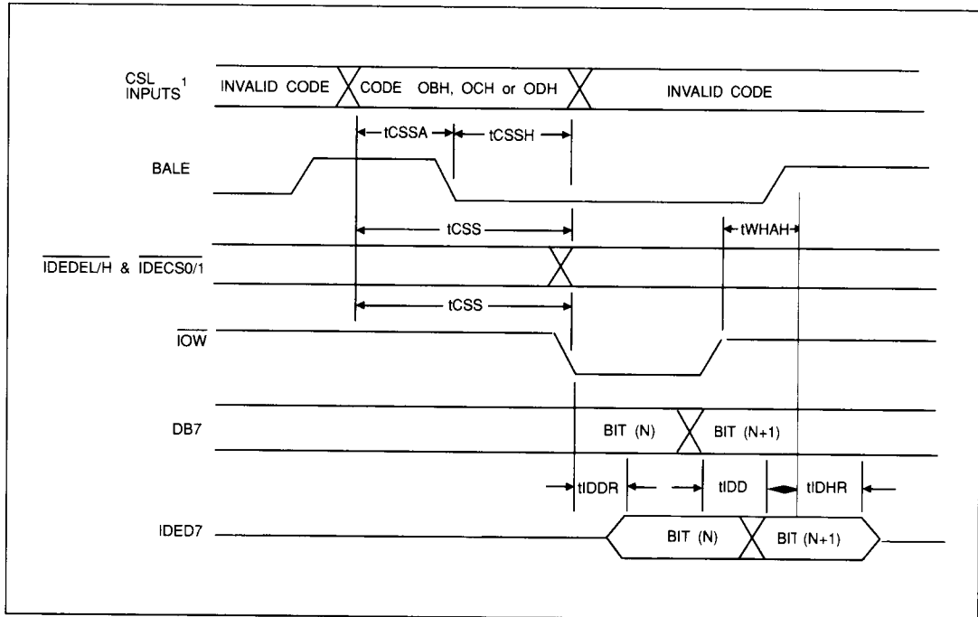
FIGURE 4-18. IDE INTERFACE W/BALE TIMING (DB7 to IDED7)
