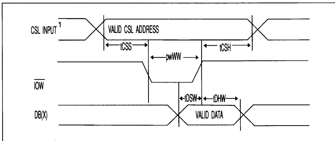
FIGURE 4-11. RTC AND RAM WRITE TIMING DIAGRAM
