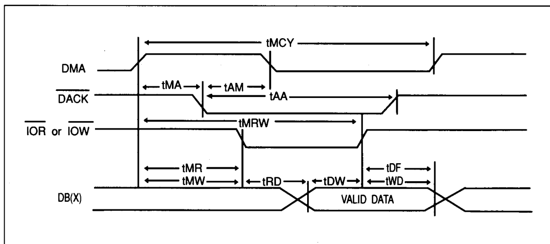
FIGURE 4-5. FDC DMA TIMING DIAGRAM
