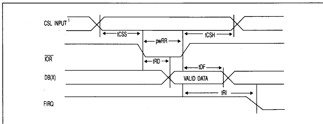
FIGURE 4-1. FDC READ TIMING DIAGRAM
