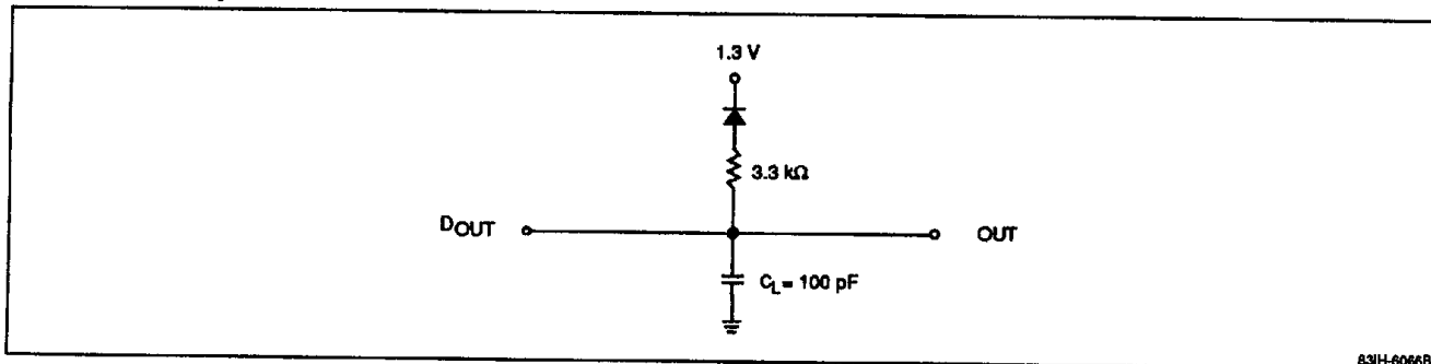
Figure 1. Output Load
