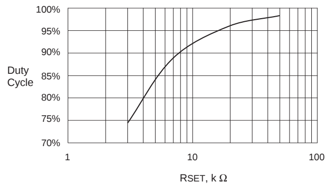
Gate Drive Maximum Duty Cycle
