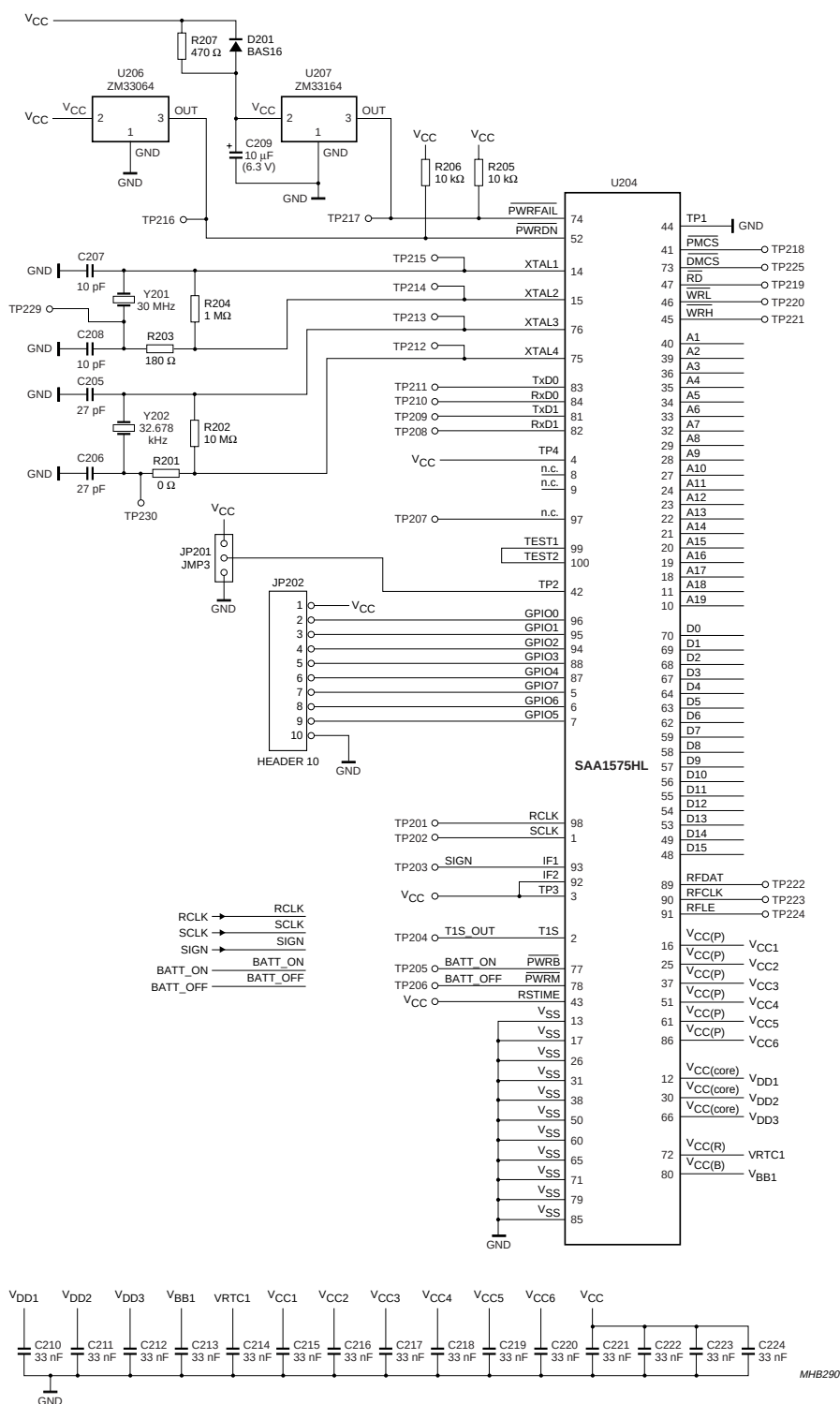
Fig.23 Baseband circuitry (continued in Fig.24).
