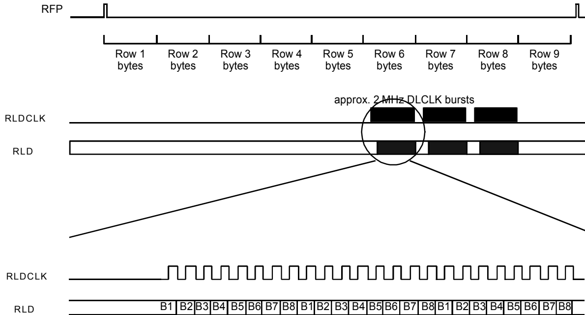
Figure 34 - Receive Line DCC Clock and Data Alignment
