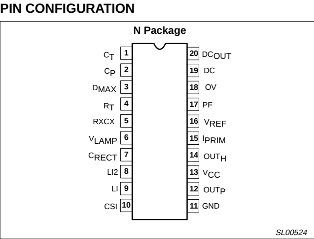
Figure 1. Pin Configuration
