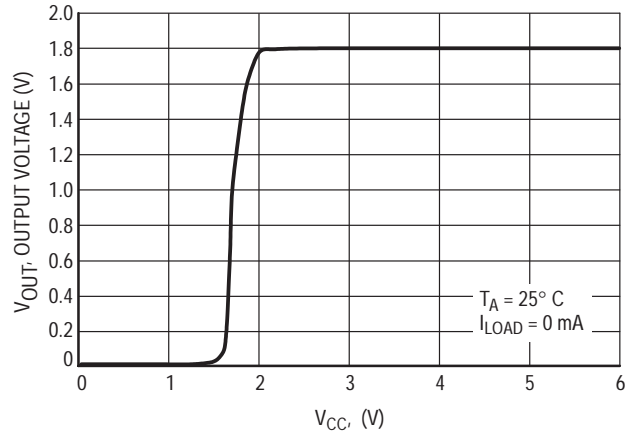
Figure 16. Output Voltage versus Input Voltage
