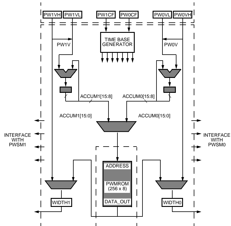
Figure 22. PWMCNTRL Architecture
