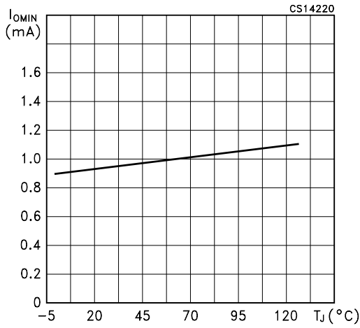
Figure 8 : Adjust Pin Current vs Temperature (Adjustable Output)
