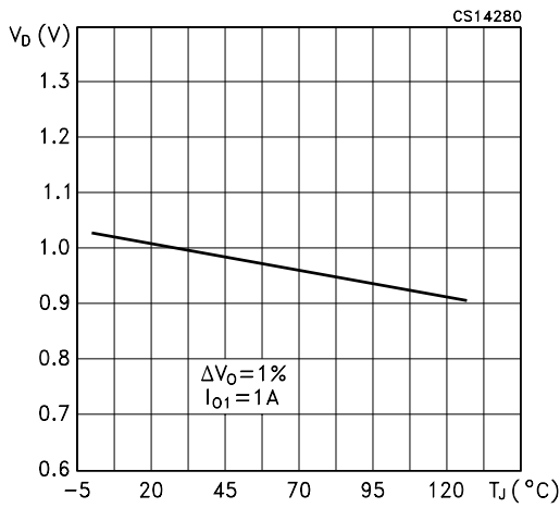
Figure 13 : Dropout Voltage vs Temperature (Fixed Output)
