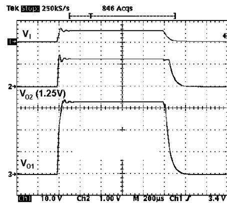
Figure 28 : Start-Up Transient
