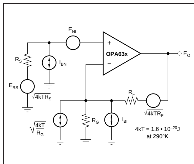
FIGURE 6. Noise Analysis Model.
