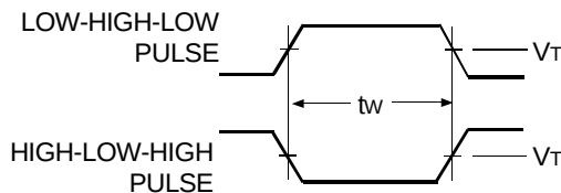
Pulse Width
