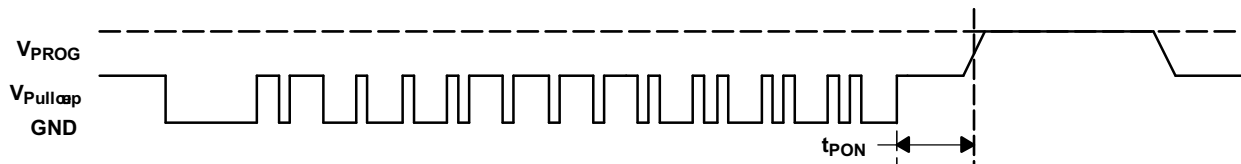
Figure 6. Writing and Programming OTP Example
