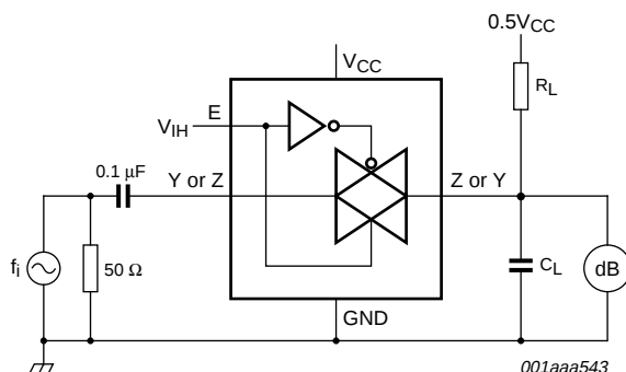
Fig 18. Test circuit for measuring the frequency response when switch is in ON-state.
