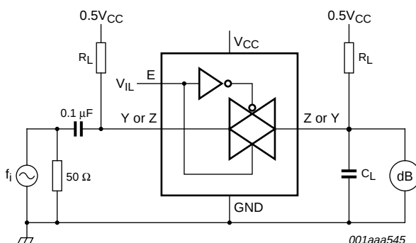
Fig 19. Test circuit for measuring feed-through attenuation when switch is in OFF-state.
