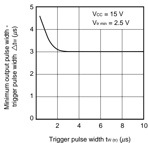
\Delta t_w - t_{tr} characteristic
