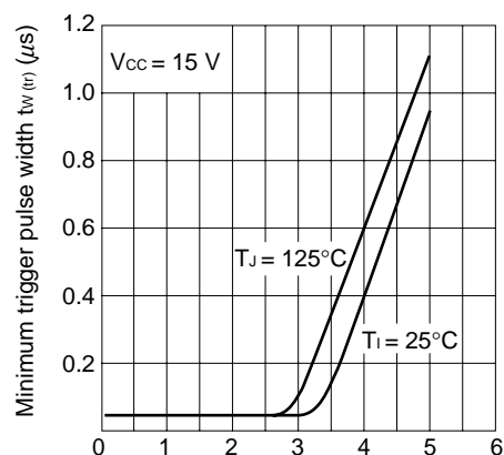
Minimum trigger pulse voltage V_{tr min.} (V)
