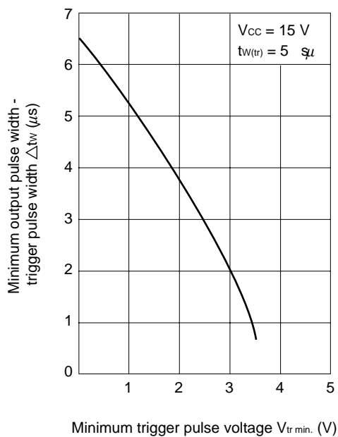
\Delta t_w - t_{tr min.} characteristic
