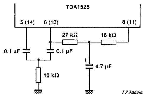
Fig.2 Double-pole low-pass filter for improved bass-boost.
