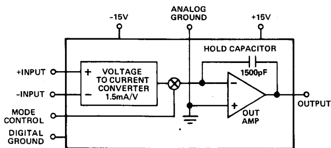
Figure 1. Block Diagram – SHA1144
