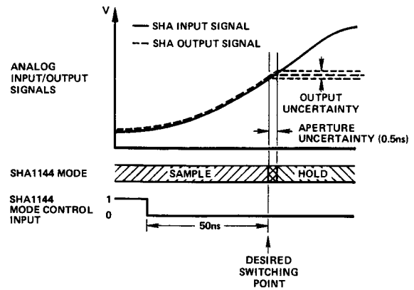
Figure 4. Aperture Uncertainty
