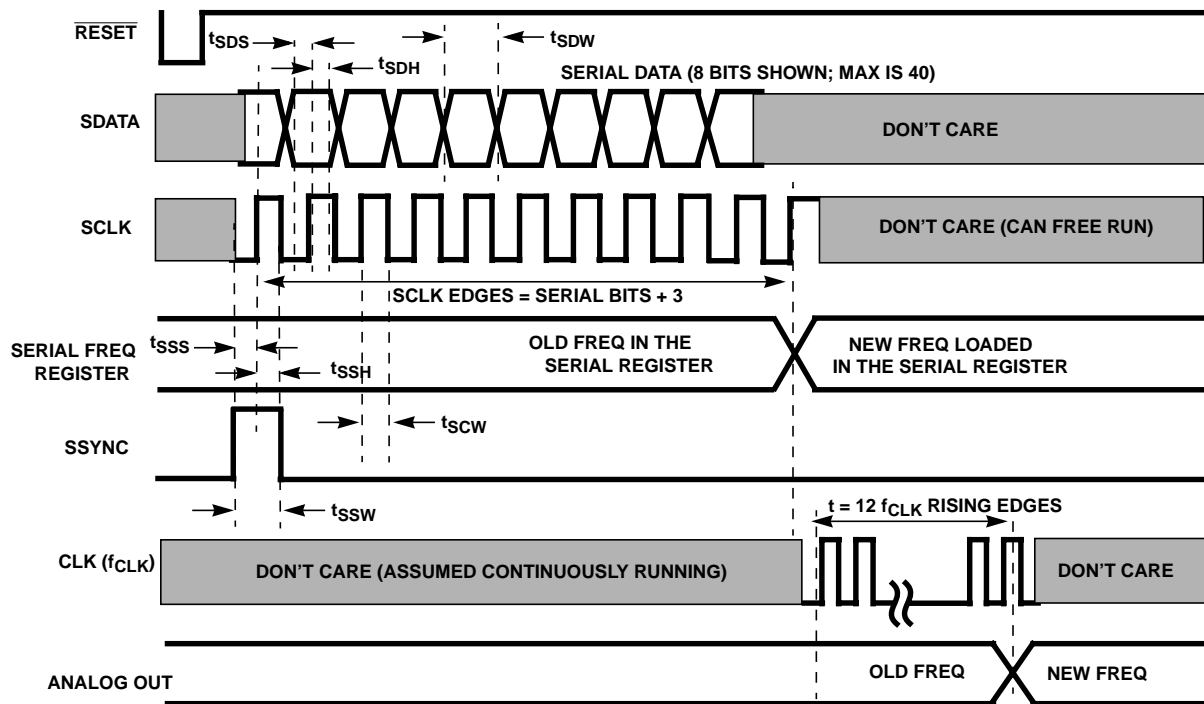
FIGURE 6. SERIAL PROGRAMMING, SYNC EARLY MODE (REPRESENTS MINIMUM SCLKS REQUIRED. SCLK CAN FREE RUN.) CONTROL REGISTER 12 IS SET TO 0001 00XX.
