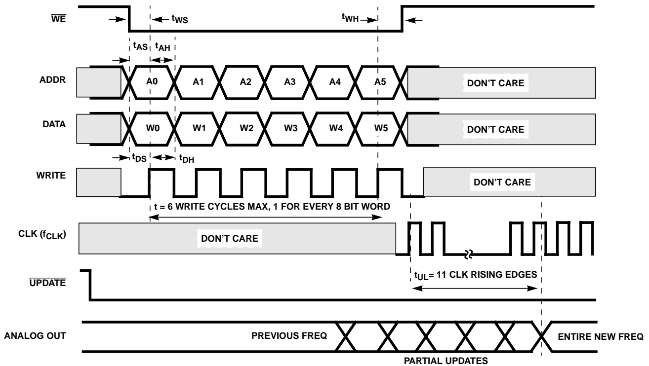
FIGURE 3. PARALLEL-LOAD METHOD 2, \overline{\text{UPDATE}} ACTIVE WHILE LOADING REGISTERS ( \overline{\text{RESET}} = \text{HIGH} )
