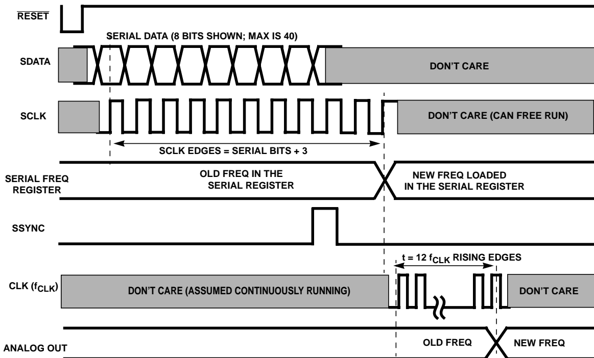
FIGURE 7. SERIAL PROGRAMMING, SYNC LATE BURST MODE (REPRESENTS MINIMUM SCLKS REQUIRED. SCLK CAN FREE RUN.) CONTROL REGISTER 12 IS SET TO 0000 00XX.
