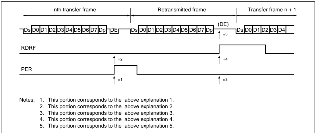
Figure 15.9 Retransmission in SCI Receive Mode
