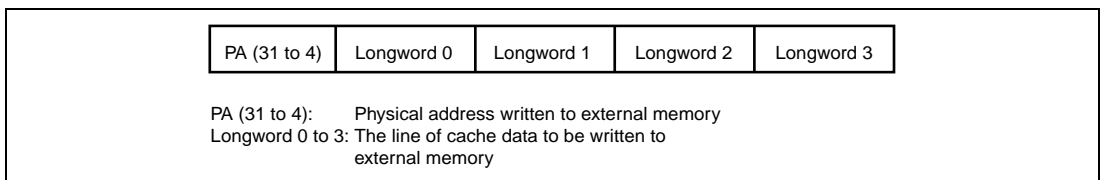
Figure 5.3 Write-Back Buffer Configuration
