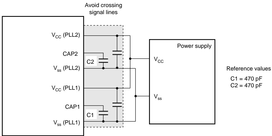
Figure 10.3 Points for Attention when Using PLL Oscillator Circuit
