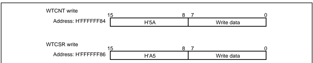
Figure 11.2 Writing to WTCNT and WTCSR
