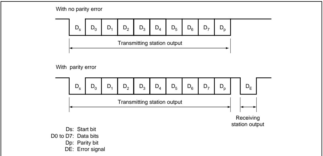
Figure 15.3 Data Format for Smart Card Interface
