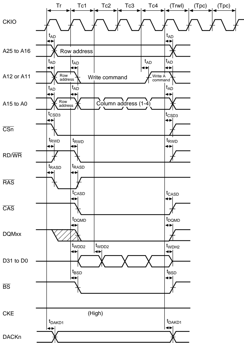
Figure 24.28 Synchronous DRAM Write Bus Cycle (Burst Mode (Single Write × 4), RCD = 0, TPC = 1, TRWL = 0)
