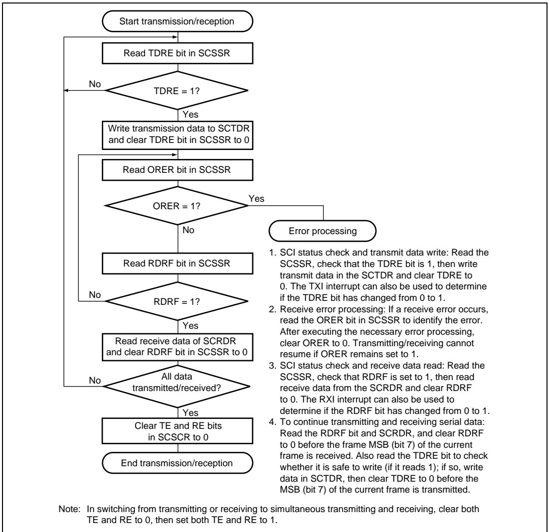
Figure 14.23 Sample Flowchart for Serial Data Transmitting/Receiving
