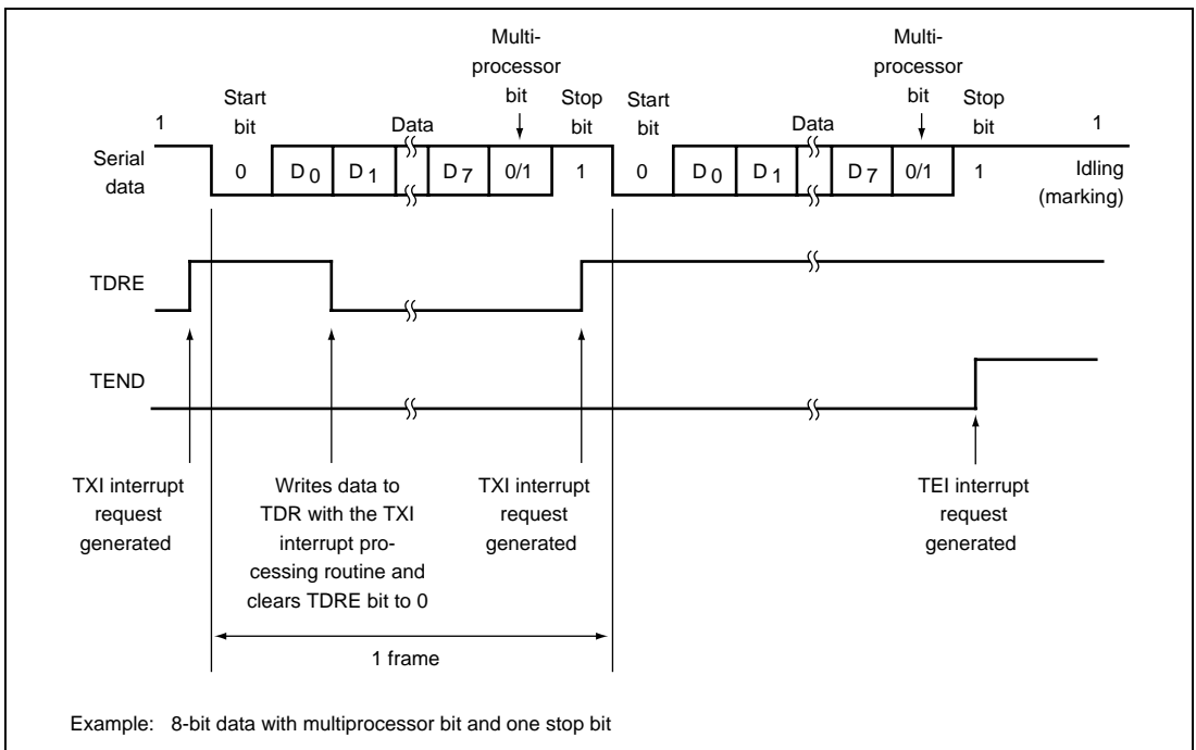
Figure 14.14 SCI Multiprocessor Transmit Operation
