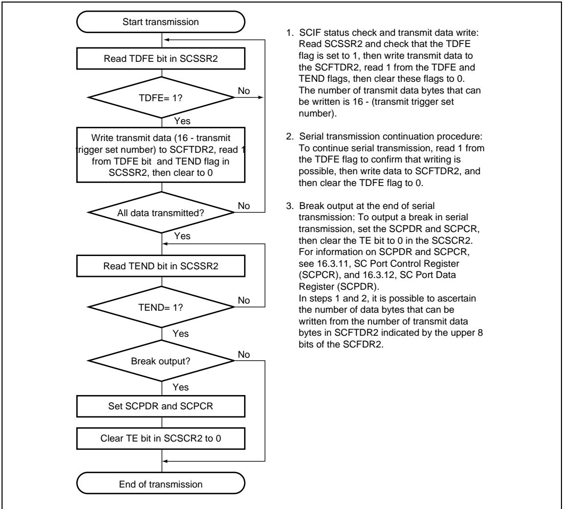
Figure 16.6 Sample Serial Transmission Flowchart
