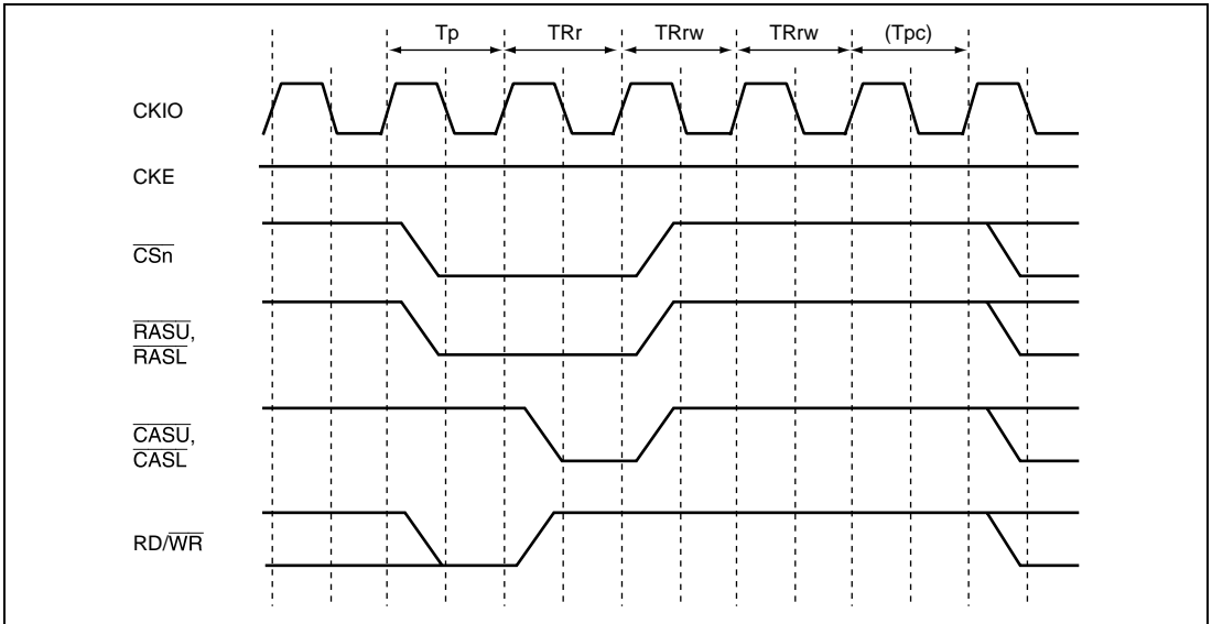
Figure 8.25 Synchronous DRAM Auto-Refresh Timing
