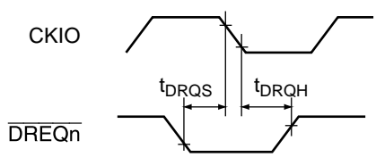
Figure 24.53 \overline{\text{DREQ}} Input Timing
