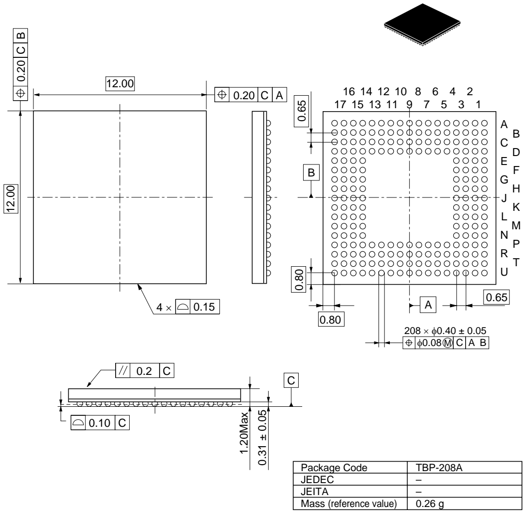
Figure D.2 Package Dimensions (TBP-208A)
