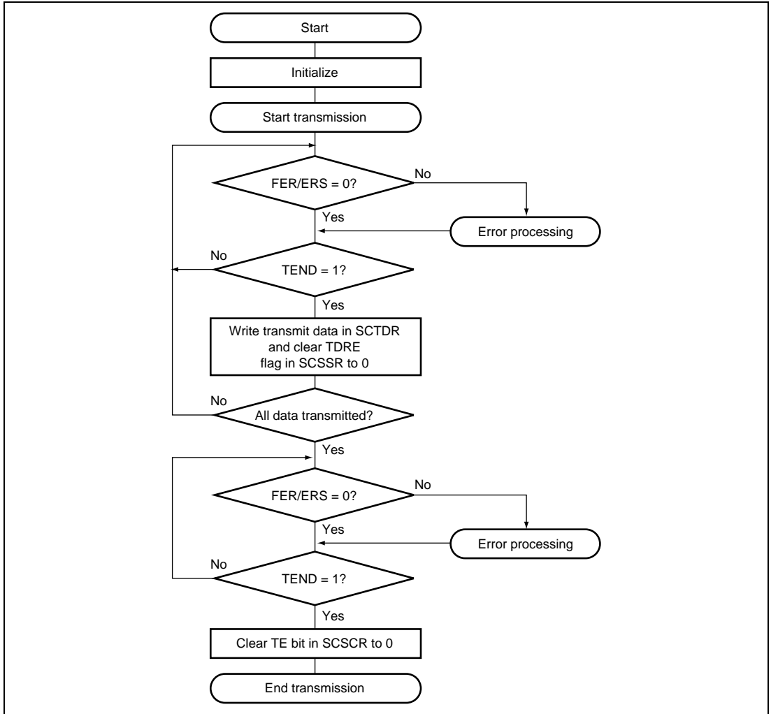
Figure 15.6 Transmission Flowchart
