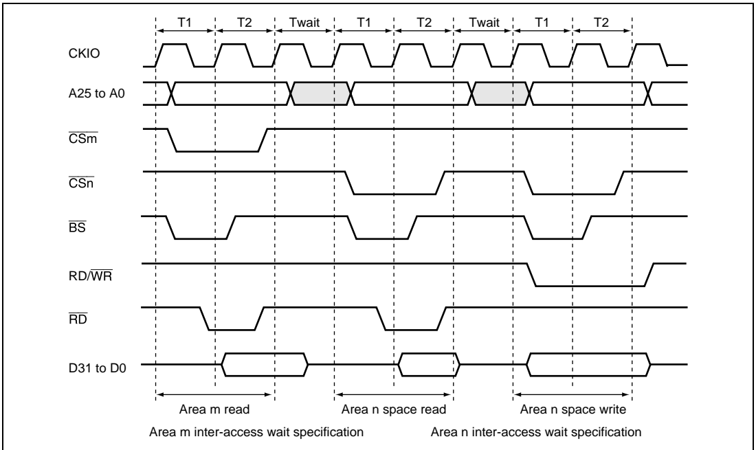
Figure 8.39 Waits between Access Cycles
