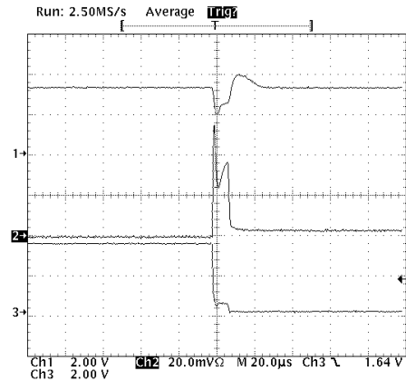
Figure 22. Short Circuit Response Time (Output Shorted to GND)
