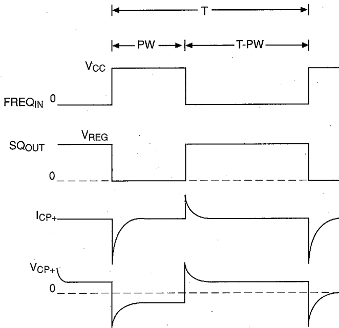
Figure 5B: Timing Diagram of FREQ_{IN} and I_{CP}
