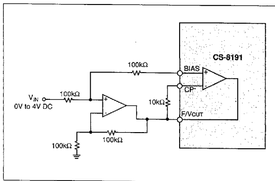
Figure 9. Driving the CS-8191 from an external DC voltage using an Op Amp Buffer.
