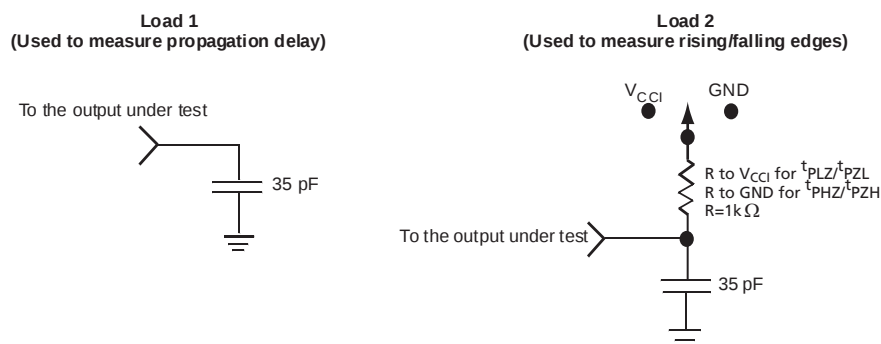
Figure 1-21 • Output Buffer Delays
