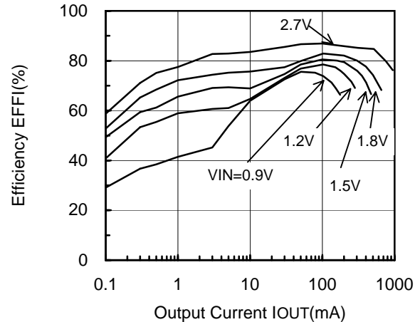
XC9104D093MR (PWM/PFM,300kHz,3.3V)
