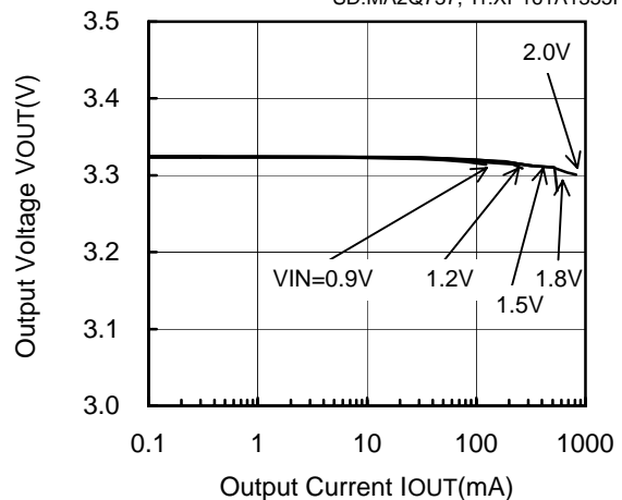
XC9104D093MR (PWM/PFM,300kHz,3.3V)
