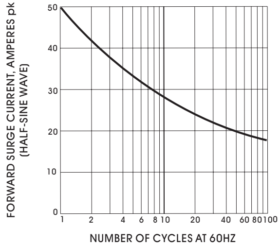
Fig.2-MAXIMUM OVERLOAD SURGE-CURRENT
