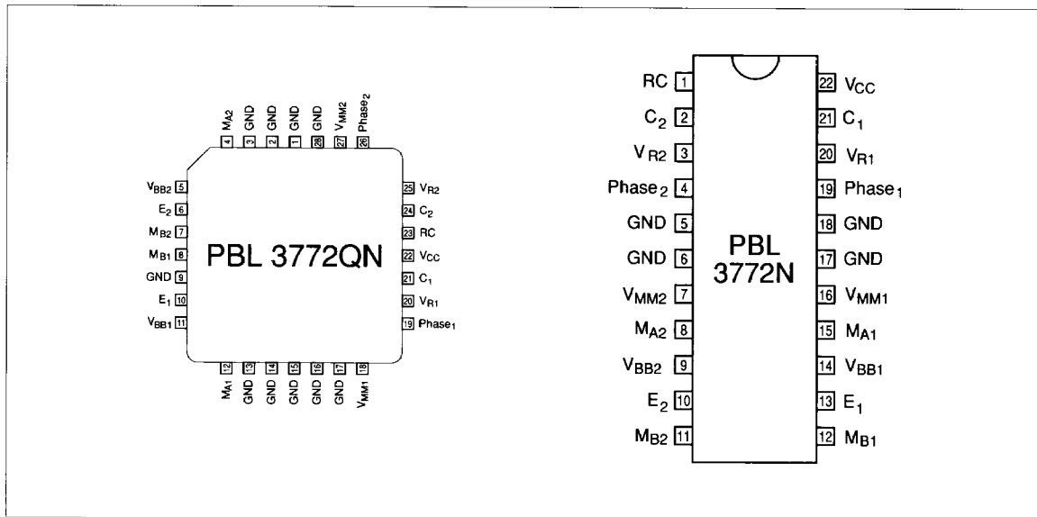
Figure 4. Pin configuration.
