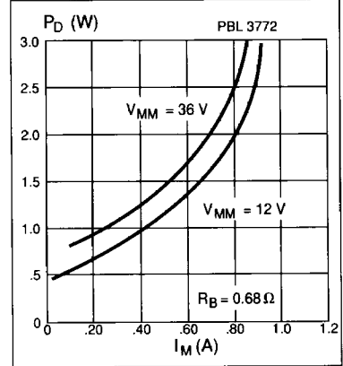
Figure 9. Power dissipation vs. motor current, both channels on. T_a = 25^\circ\text{C} .
