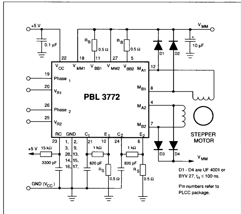
Figure 6. Typical stepper motor driver application with PBL 3772.
