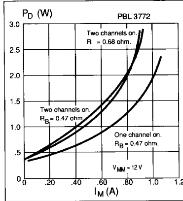
Figure 8. Power dissipation vs. motor current. T_a = 25^\circ\text{C} .
