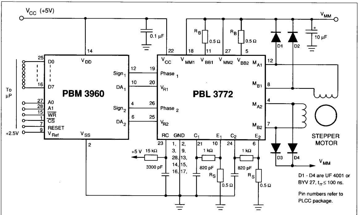
Figure 7. Microstepping system with PBM 3960 and PBL 3772.
