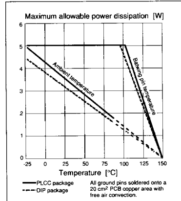
Figure 10. Maximum allowable power dissipation vs. temperature.
