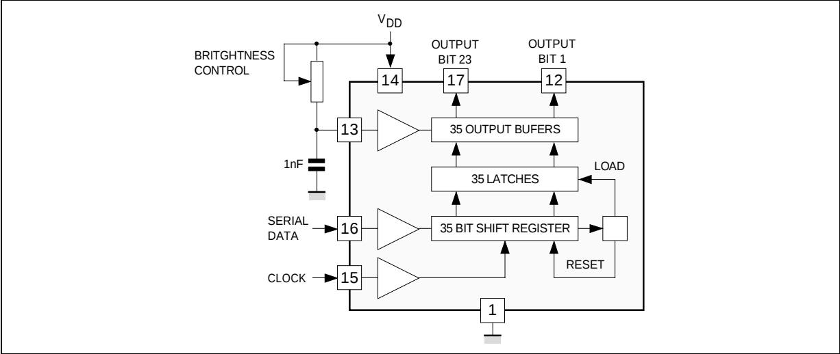
BLOCK DIAGRAM (Figure 1)
