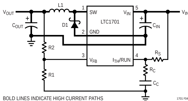
Figure 4. LTC1701 Layout Diagram (See Board Layout Checklist)
