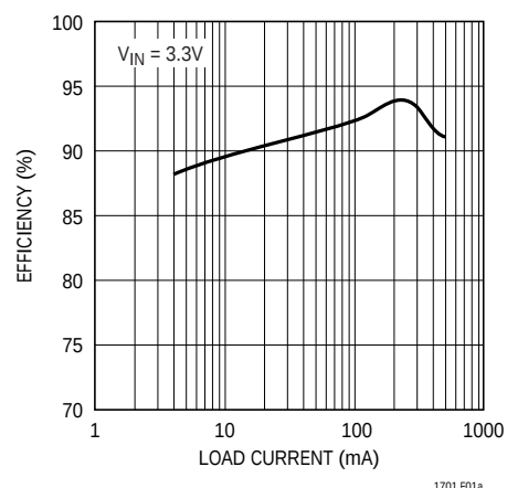
Efficiency Curve
