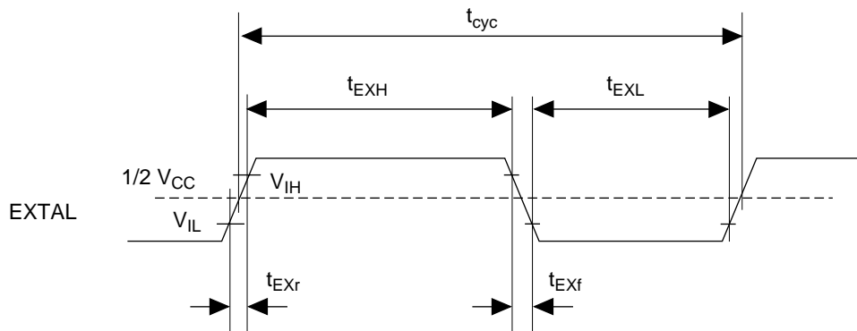
Figure 20.45 EXTAL Input Timing
