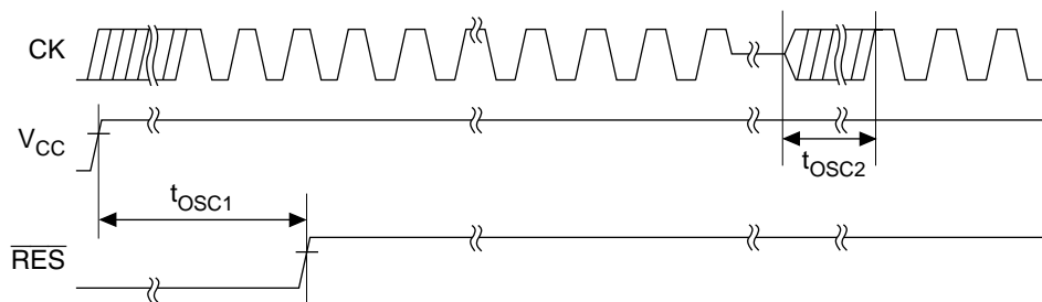
Figure 20.47 Oscillation Settling Time
