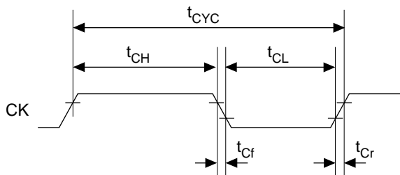
Figure 20.46 System Clock Timing
