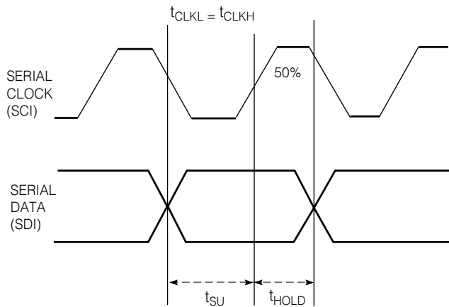
Fig. 7 Waveforms
