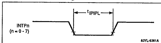
Figure 27. ICU Timing
