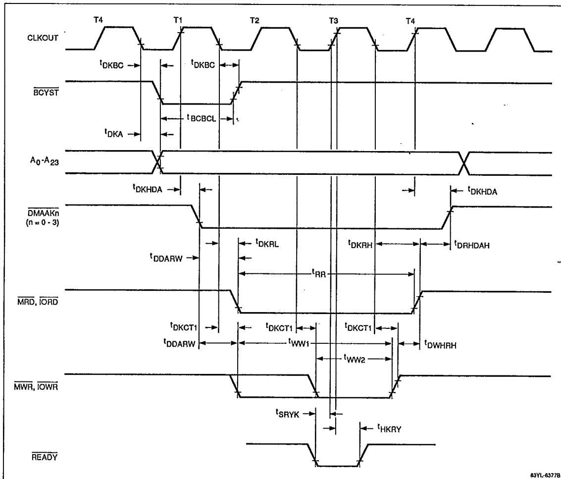
Figure 23. DMA Timing 1
