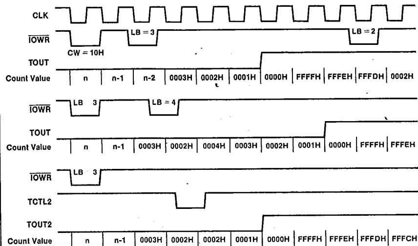
Figure 69. Timer Counter Unit (TCU) Waveforms (Sheet 1 of 3)
