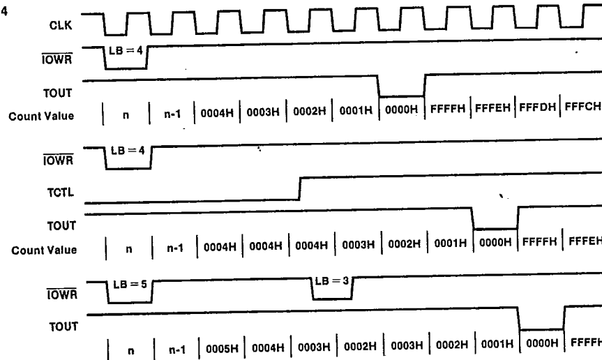
Figure 69. Timer Counter Unit (TCU) Waveforms (Sheet 3 of 3)
