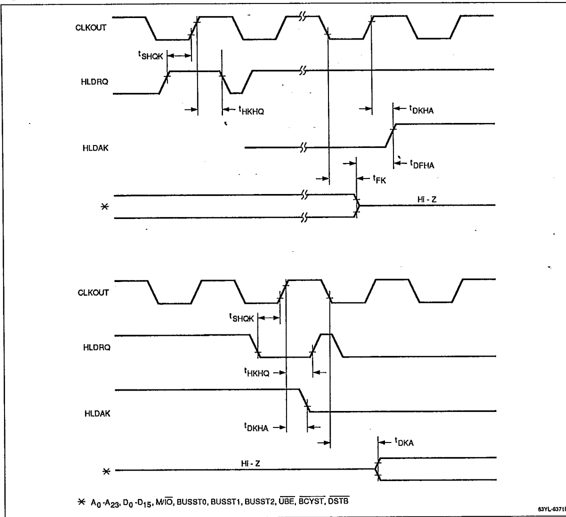
Figure 17. Bus Hold
