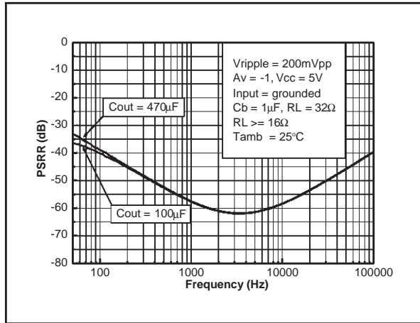
Fig. 55: PSRR vs Output Capacitor
