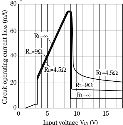
Fig.18 Circuit Operating Current vs. Input Voltage (PQ09RF2/PQ09RF21/PQ09RF2V)
