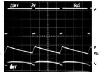
STEP-DOWN CONVERSION
