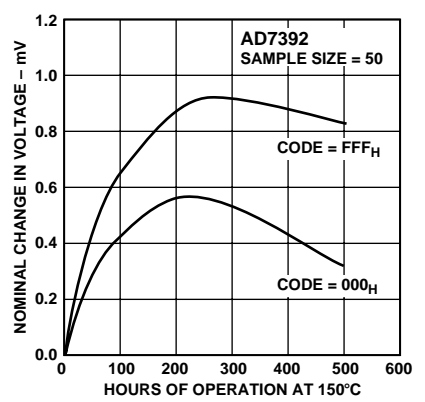
Figure 22. Long-Term Drift Accelerated by Burn-in
