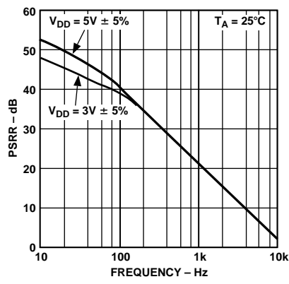
Figure 15. Power Supply Rejection vs. Frequency
