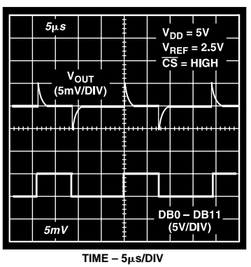
Figure 18. Digital Feedthrough
