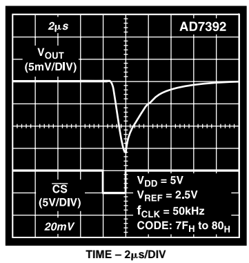
Figure 17. Midscale Transition Performance
