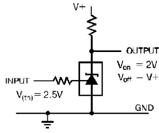
FIGURE 2. SINGLE-SUPPLY COMPARATOR WITH TEMPERATURE-COMPENSATED THRESHOLD
