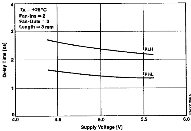
Delay Time vs Supply Voltage [NAND]
