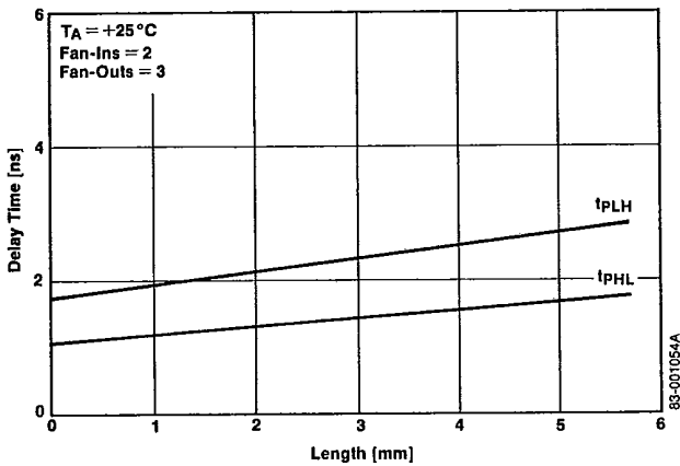
Delay Time vs Length [NAND]
