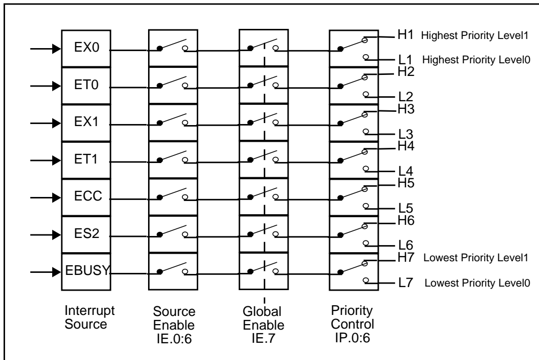
Figure 13 Interrupt Structure
