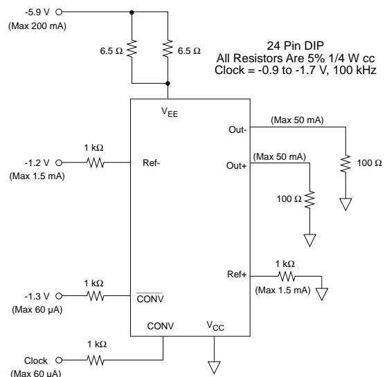
Figure 7 - Burn-In Circuit
