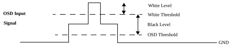
Figure 11 - OSD Input Signal Waveform
