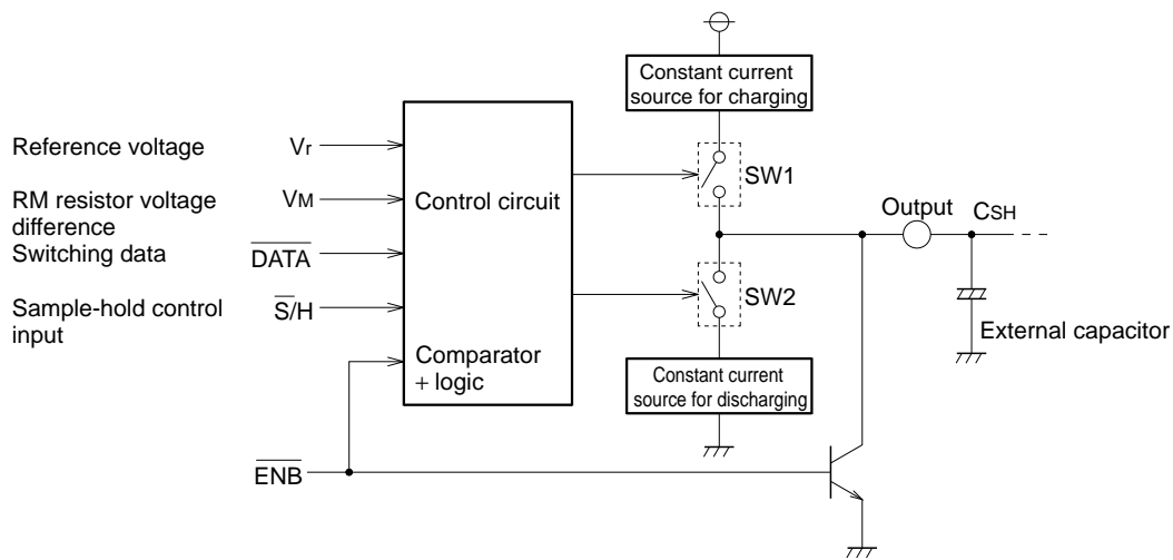
Conceptual Diagram: Sample-Hold Circuit
