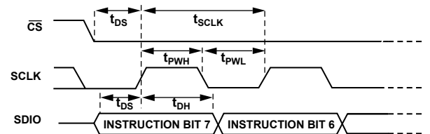
Figure 11. Timing Diagram for Register Write to AD9725
