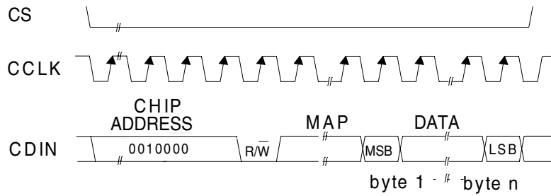
Figure 8. Control Port Timing, SPI Format
