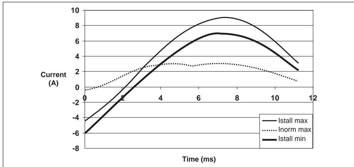
Fig. 8: Motor current maximum ranges
