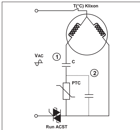
Fig. 1: One-triac topology
