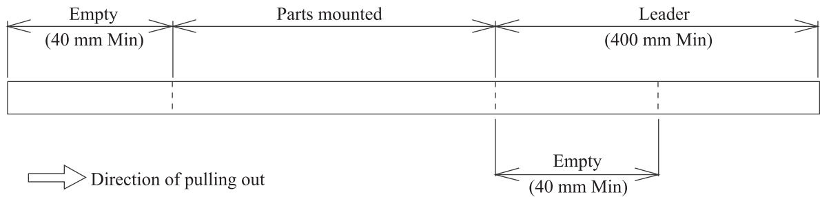
Figure 12. ZHX1810 Tape Dimensions and Configuration (Unit: mm)
